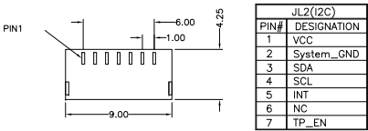
DETAIL B
