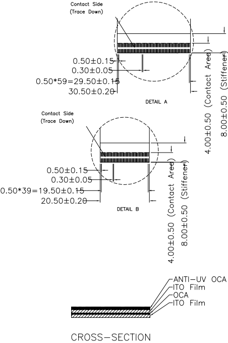
CROSS-SECTION
