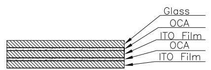
CROSS-SECTION
