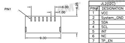
DETAIL B
