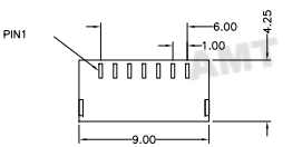
DETAIL B
