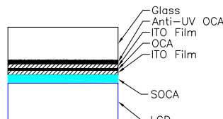
CROSS-SECTION
