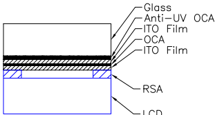
CROSS-SECTION
