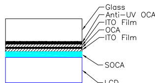
CROSS-SECTION
