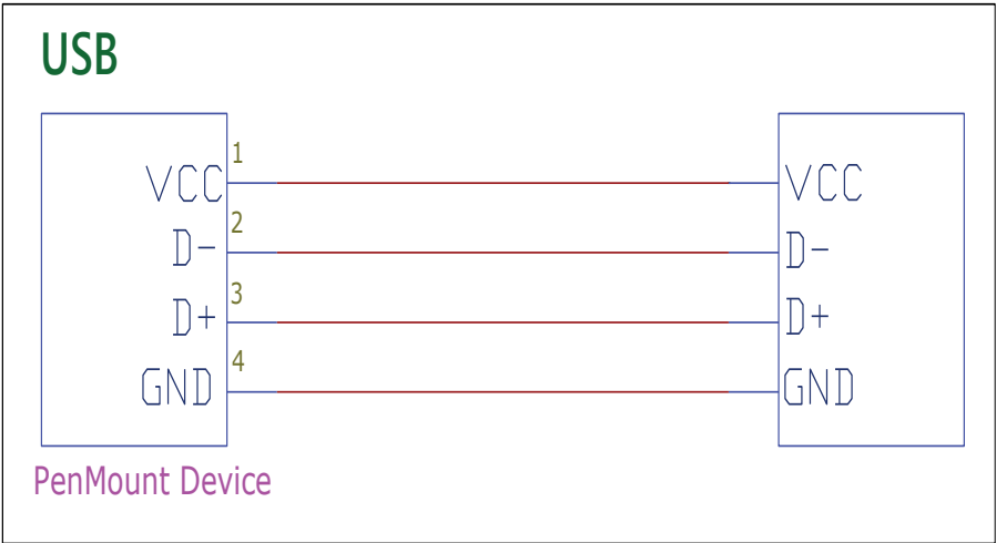
Figure 3. USB interface
