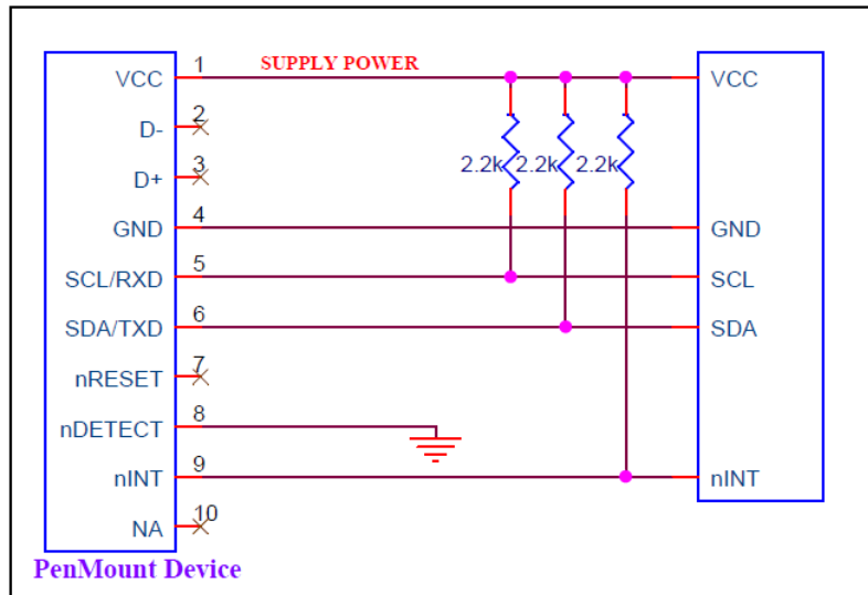
Figure 3. I2C interface
