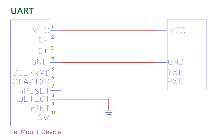
Figure 2. UART interface
